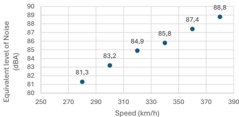
Fig.10. Increase in noise level as a function of speed [25]
