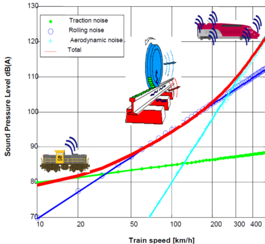
Fig. 6. Noise sources as a function of speed [4]
